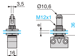
ZCE06
