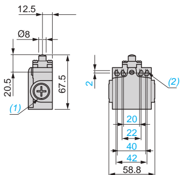
XCNT2●10P16
