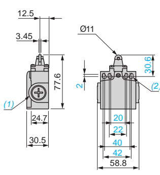
XCNT2●02P16
