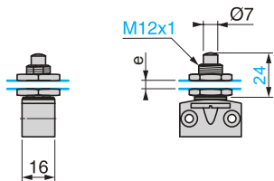
ZCEF0
