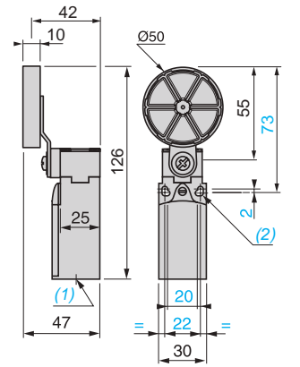
XCKN2●39P20
