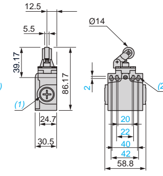
XCNT2●21P16
