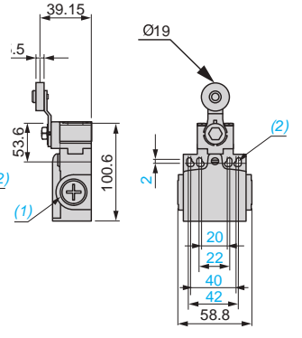
XCNT2●18P16
